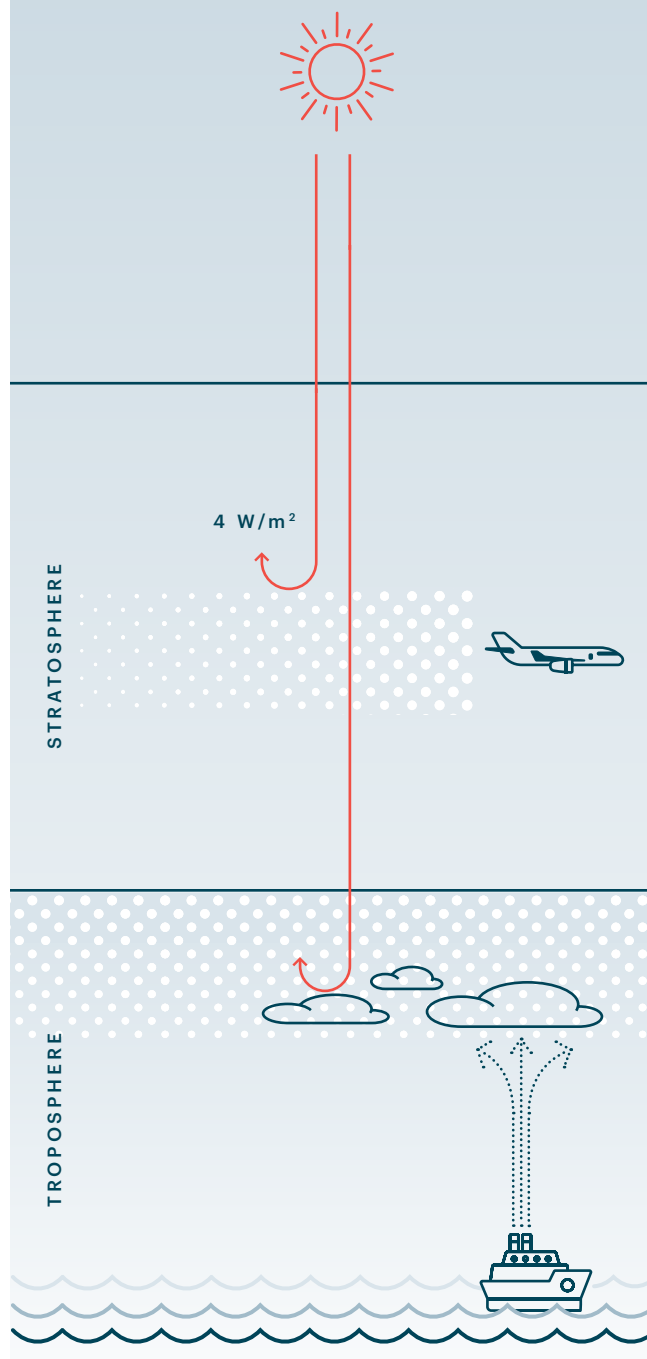
FIGURE 4. APPROACHES TO INCREASING THE REFLECTION OF SUNLIGHT FROM THE ATMOSPHERE.
