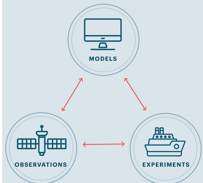
FIGURE 13. CLIMATE INTERVENTION RESEARCH.
